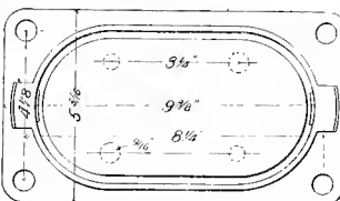
Figs. 5190-5191. KING'S YIELDING SIDE-BEARING.
